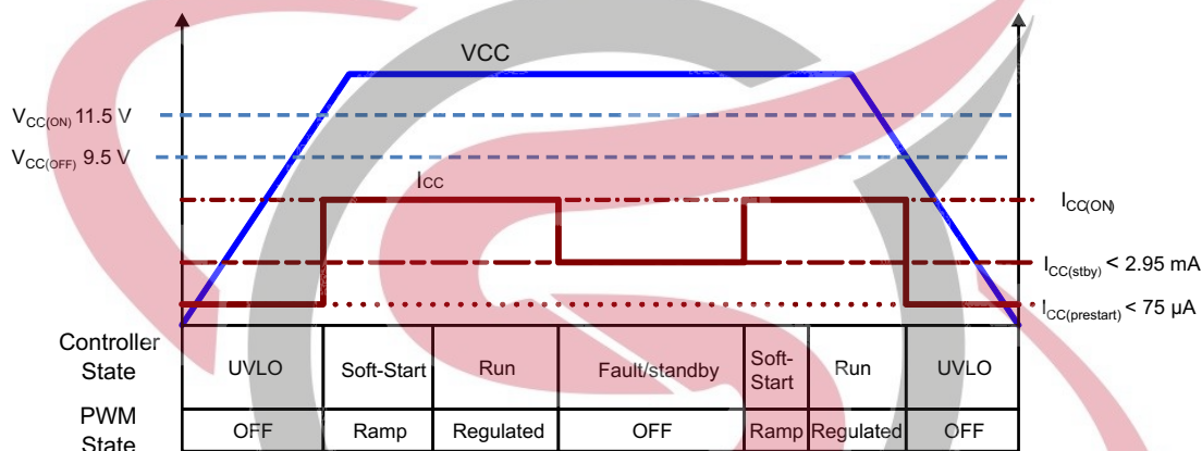
Figure 40. Device Supply States
